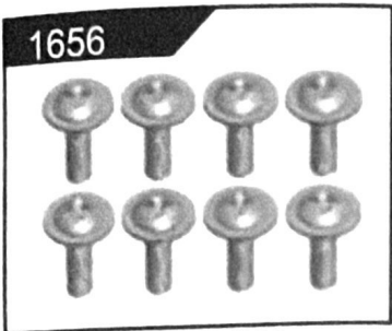
2.5*8PWM6 Cross round head machine screw 十字圆头ST2.5*8PWM6 碳钢 镀黑锌组
